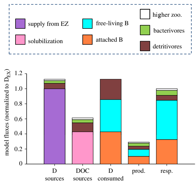
Fig. 2. Model results for standard parameter settings (Table 1), normalized to detritus input from the euphotic zone ( D_{EX} ): detritus (D) sources, DOC sources, detritus consumption (in the case of free-living bacteria via solubilization to DOC), production and respiration. EZ, euphotic zone; B, bacteria; zoo., zooplankton.
