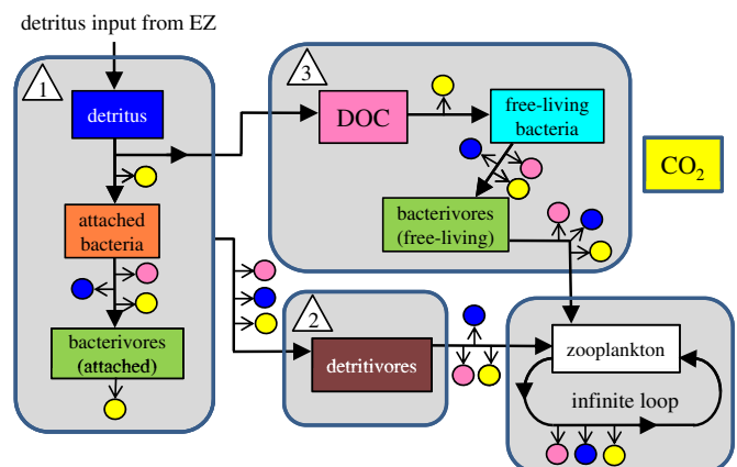
Fig. 1. Flow diagram of model. Detritus input from the euphotic zone (EZ) is cycled through the mesopelagic food web via POC (dark blue fluxes) and DOC (pink fluxes) and is ultimately respired as CO_2 (yellow fluxes); fluxes to small colored circles enter either detritus, DOC or CO_2 , according to color code. The three main food web pathways are (1) via attached bacteria, (2) via detritivores and (3) via DOC and free-living bacteria (see text).
