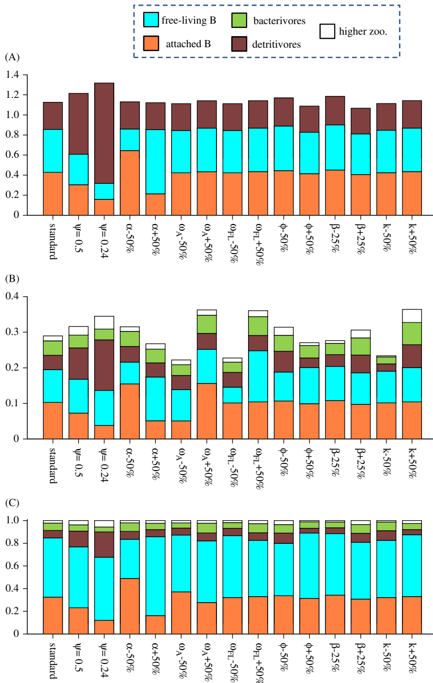
Fig. 3. Model sensitivity to parameters: (A) consumption of detritus, (B) production, (C) respiration. Parameters for zooplankton (detritivores, bacterivores, higher predators), \phi , \beta and k , were varied simultaneously. Results are normalized to detritus input from the euphotic zone ( D_{EX} ). B, bacteria; zoo., zooplankton. See Table 1. for key of model parameters.
