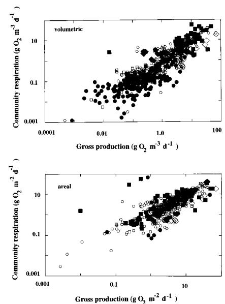
Fig. 2. The relation between volumetric and areal rates of community respiration rate and gross primary production in aquatic ecosystems ( \square , lakes; \blacksquare , rivers; \diamond , marshes; \circ , coastal systems; \bullet , open sea).
