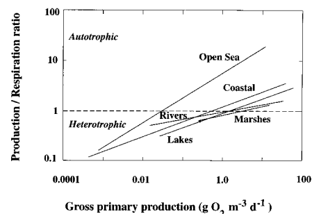
Fig. 3. Regression lines describing the relation between the ratio of gross primary production to respiration rate and the gross primary production of different aquatic ecosystems.
