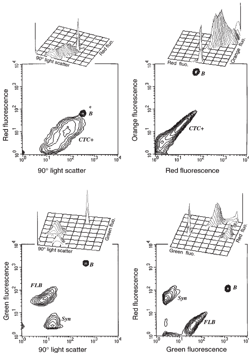
FIG.8. – Upper panels. Flow cytometric analysis of a Mediterranean plankton sample after incubation with 5 mM CTC for a few hours showing the presence of a bacterial population that took up the fluorescent CTC (labeled as CTC+). Yellow beads (B) were included in the run. The panels present contour density plots of 10000 acquired events. In the left side of the graphs, a representation of 90° light scatter (SSC) vs. red fluorescence (FL3). In the right side, a representation of orange fluorescence (FL2) vs. red fluorescence. Note that the 3-D representation of the FL2 vs. FL3 plot has been turned around to better show that the main peak is separated from the background. Lower panels. Flow cytometric signature of FITC-stained Pseudomonas diminuta (FLB) added as a tracer for grazer experiments to a Mediterranean plankton sample particularly rich in Synechococcus (labeled as Syn). Yellow beads (B) were included in the run. The panels present contour density plots of 10000 acquired events. In the left side of the graphs, a representation of 90° light scatter (SSC) vs. green fluorescence (FL1). In the right side, a representation of red fluorescence (FL3) vs. green fluorescence. Note that the 3-D representation of the FL1 vs. FL3 plot has been turned around to better show the separation of both populations.
