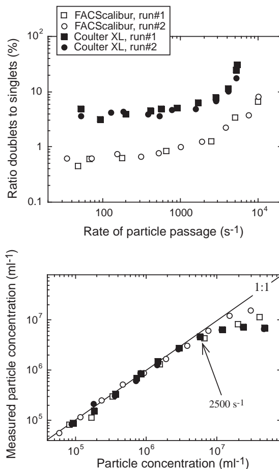
FIG. 4. – Effects of the speed of particle passage through two different flow cytometers (Coulter XL and Becton and Dickinson’s FACSscalibur). The speed was changed by serially diluting a fluorescent bead solution: Upper panel, the amount of beads detected as doublets. Lower panels, relationship between the actual particle concentration and the flow cytometrically measured particle concentration.
