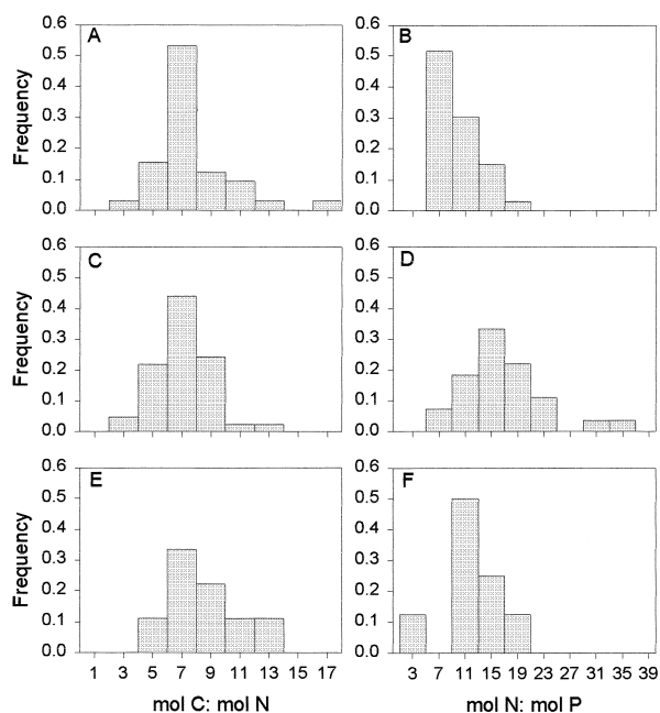
Fig. 1. Elemental composition of (A, B) nutrient-replete marine microalgal and cyanobacterial cultures, (C, D) marine particulate matter and (E, F) nutrient draw-down during phytoplankton blooms. (C)–(F) should be interpreted with caution as no attempt was made to ensure that the samples summarized here are representative of the ocean as a whole. Rather, the oceanographic observations reflect the data base that is available in the literature. Sources of information for phytoplankton cultures are Burkhardt et al. (1999), Goldman et al. (1992), La Roche et al. (1993), Nielsen (1992, 1996), Parsons et al. (1961), Sakshaug et al. (1983, 1984), Terry et al. (1983). Sources of information for marine particles are Arrigo et al. (1999), Banse (1974) citing data of Antia et al. (1963), Bishop et al. (1977, 1980), Christian & Lewis (1997), Copin-Montegut & Copin-Montegut (1983), Daly et al. (1999), Eppley et al. (1977, 1988, 1992), Fraga (1966), Herbland & Le Bouteiller (1983), Herbland et al. (1998), Karl et al. (1995), Menzel & Ryther (1966), Perry (1976), Rios et al. (1998), Sakshaug & Holm-Hansen (1986), Tanoue (1985), Tréguer et al. (1988). Sources of information for nutrient draw-downs are Arrigo et al. (1999), Banse (1974), Codispotti et al. (1986), Cooper (1933a, b), de Baar et al. (1997), Haigh et al. (1992), Rubin et al. (1998), Sambrotto & Langdon (1994), Turner & Owens (1995), van Leeuwe et al. (1997), Wallace et al. (1995). The number of observations included in the histograms is as follows (A) 34, (B) 34, (C) 41, (D) 27, (E) 8, (F) 8. Only reports that presented C, N and P contents were included in panels (A) and (B).
