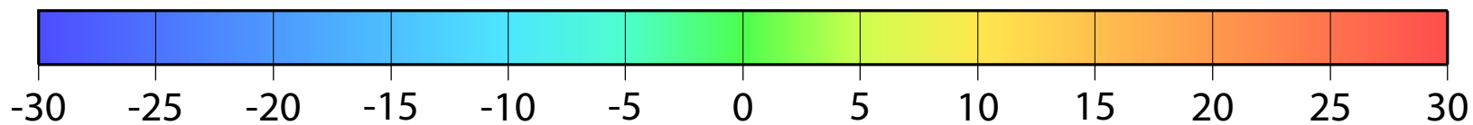
Sea Surface Height Anomaly (cm)
