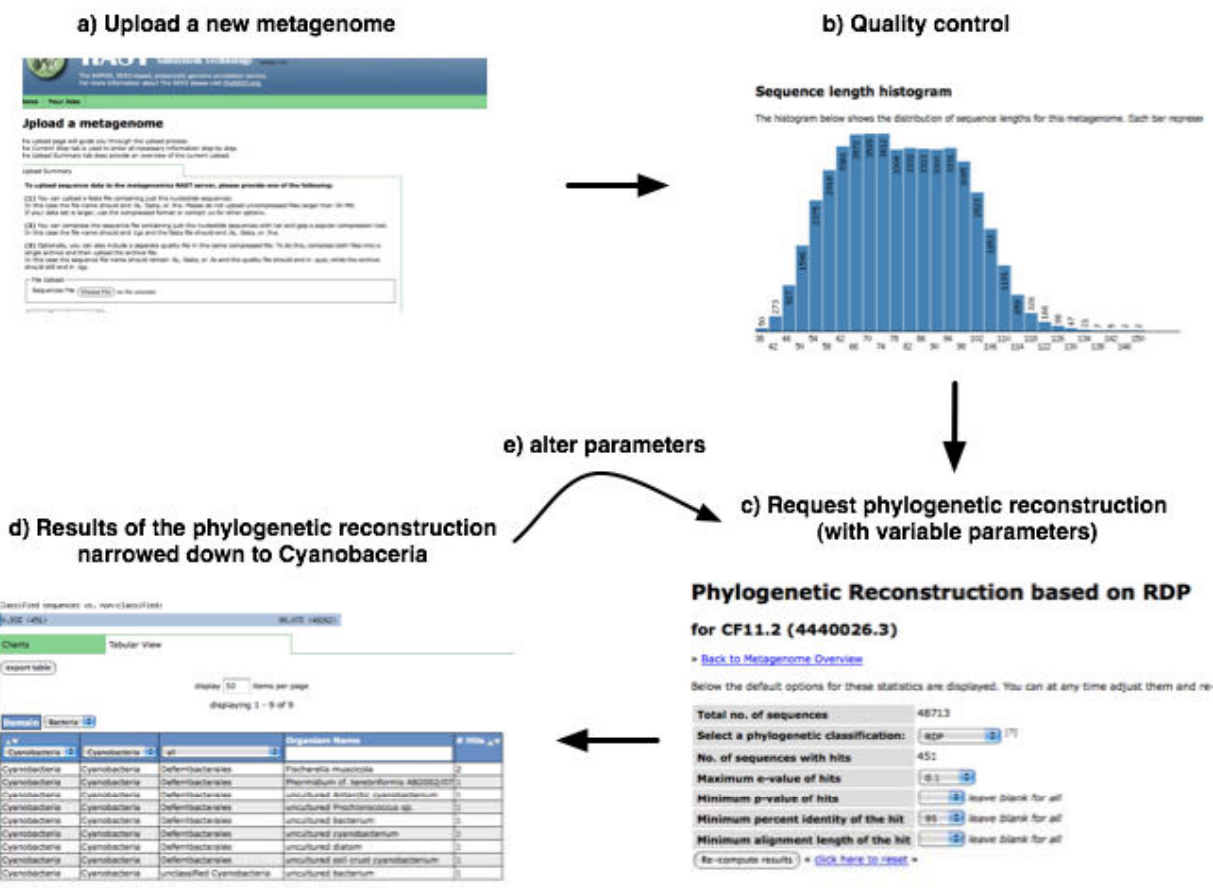
Figure 1 After uploading a dataset (a), the system computes initial quality control (b) and allows the user to set the parameters for phylogenetic analysis (c). The system then displays the results (d) and allows the user to alter the parameters (e). Data shown in this example is from the dataset CF11.2 (ID:4440026.3) that is publicly available in the MG-RAST server.
