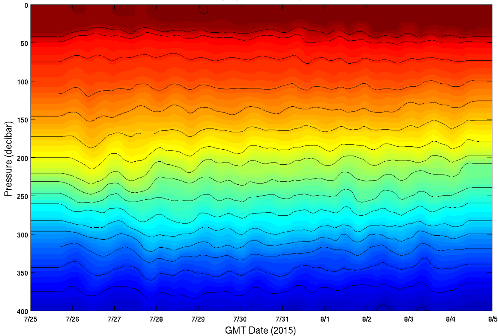
HOE-Legacy 2A, CTD Temperature
