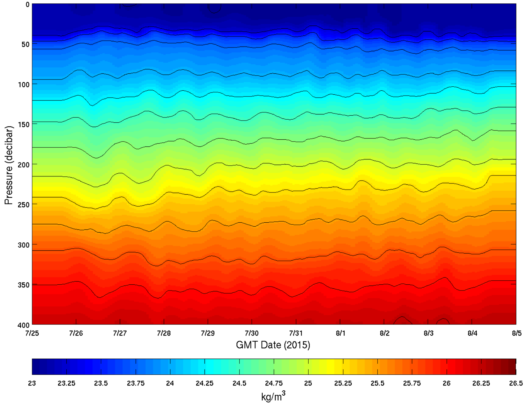
HOE-Legacy 2A, CTD Potential Density
