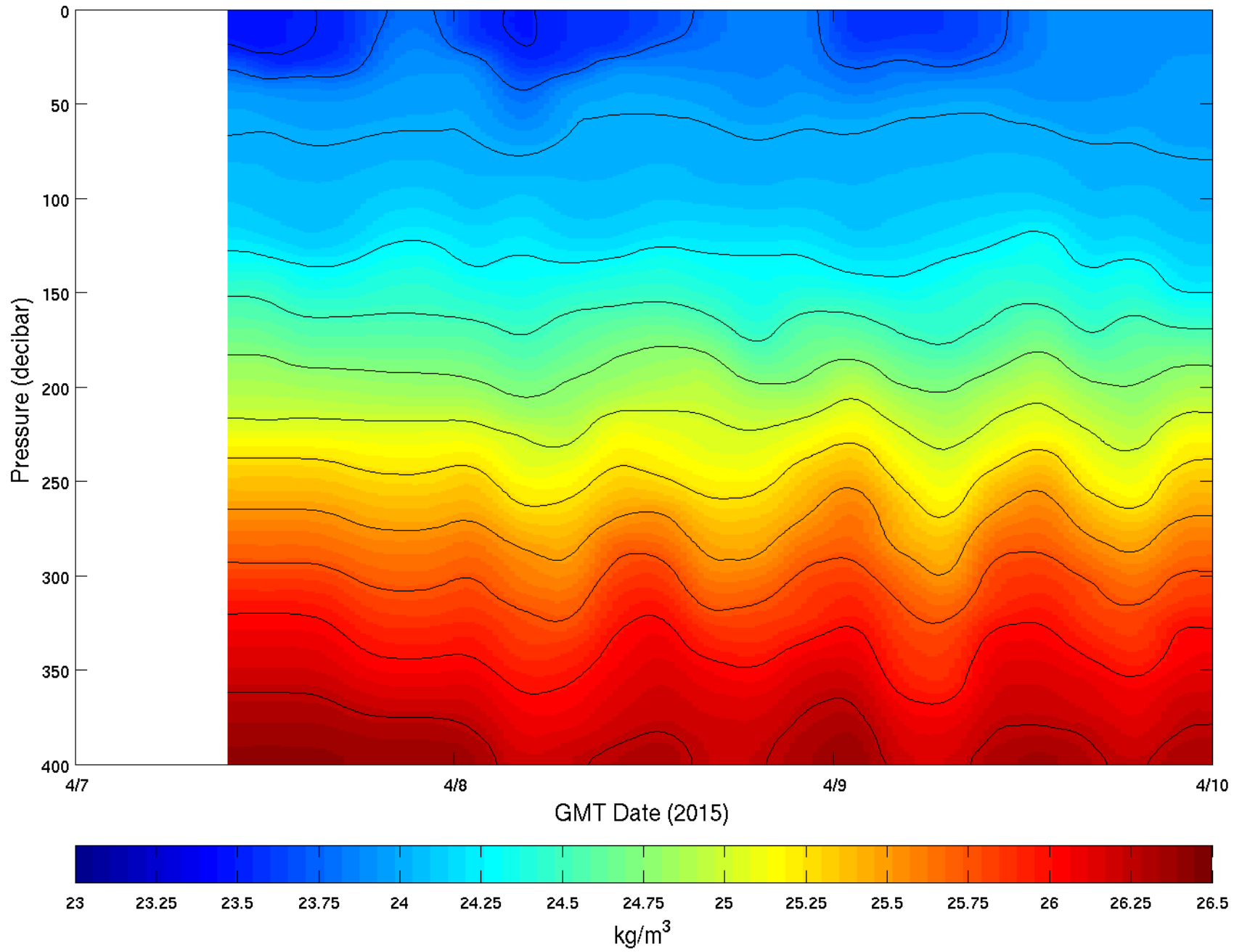
HOE-Legacy 1, CTD Potential Density
